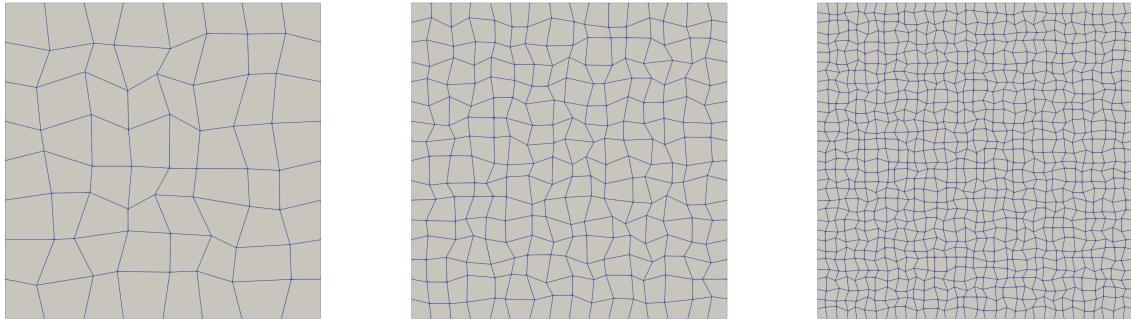
Figure 1: Example of non-nested multigrid levels.
